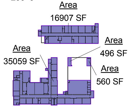
④ Level 3 1" = 200'-0"
